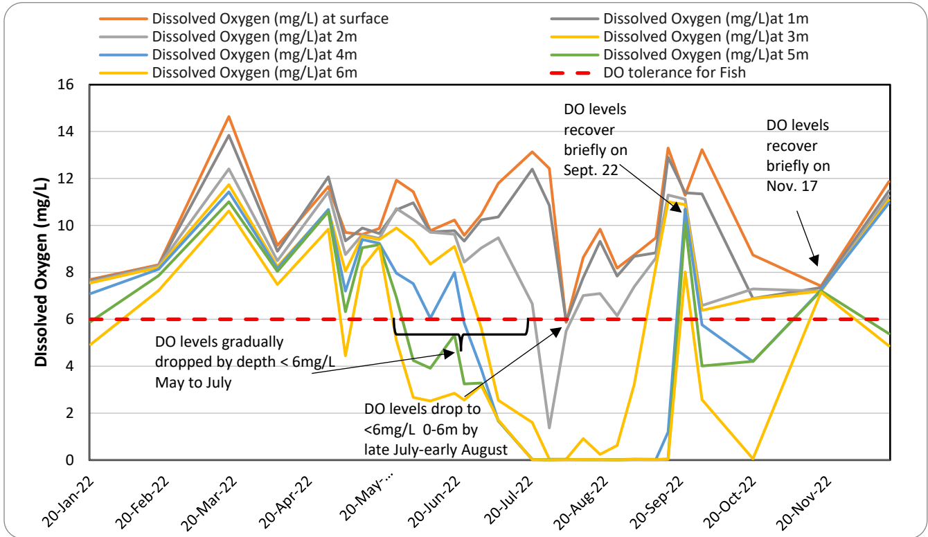
Chart 2: Somenos Lake Water Quality Profile and Dissolved Oxygen Tolerance for Salmon
