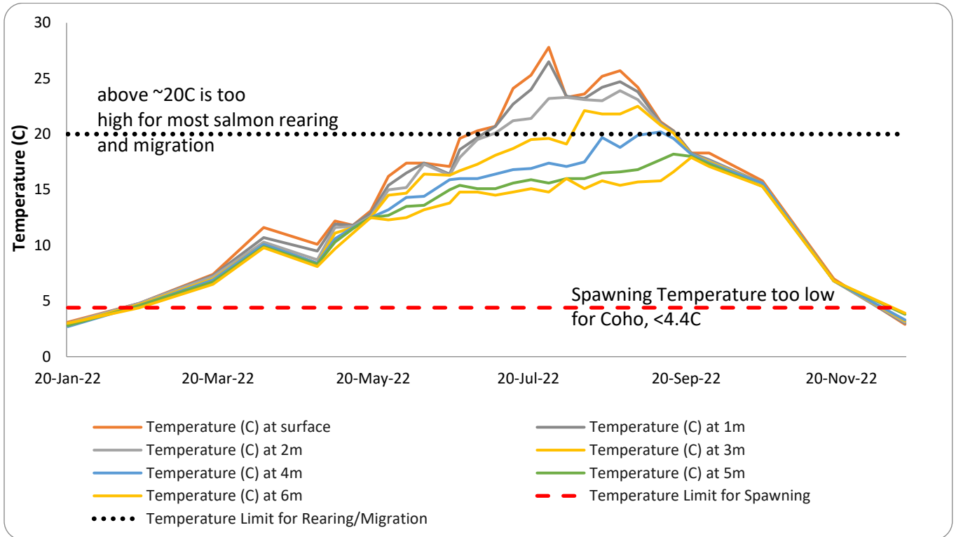
Chart 3: Somenos Lake Water Quality Profile and Temperature Tolerance for Salmon
